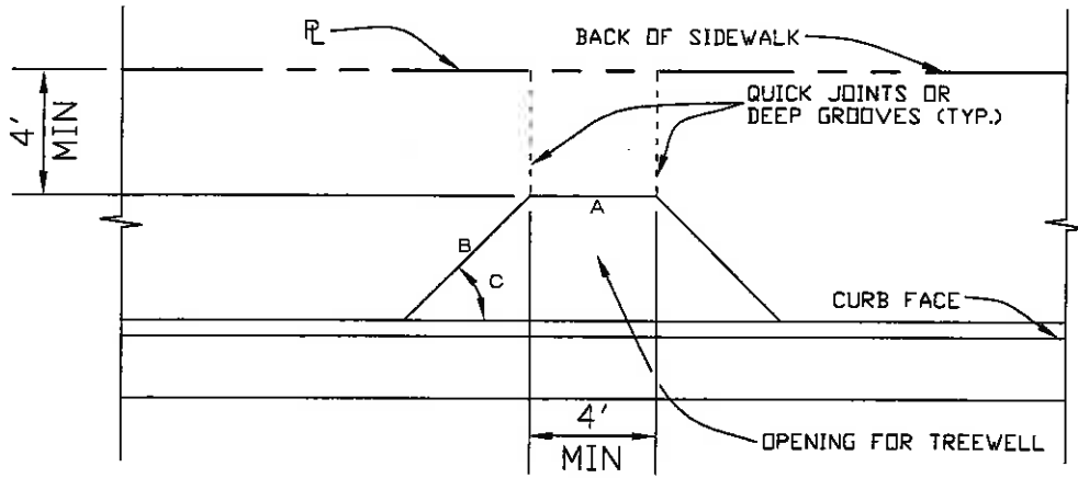
FULL WIDTH SIDEWALK
