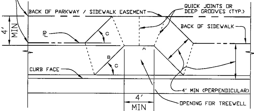
OFFSET SIDEWALK CASE I
