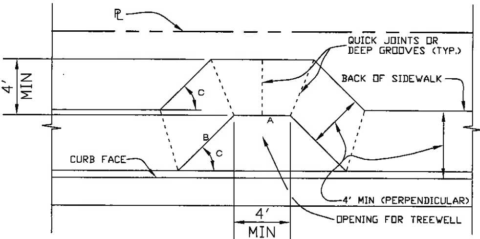
OFFSET SIDEWALK CASE II
