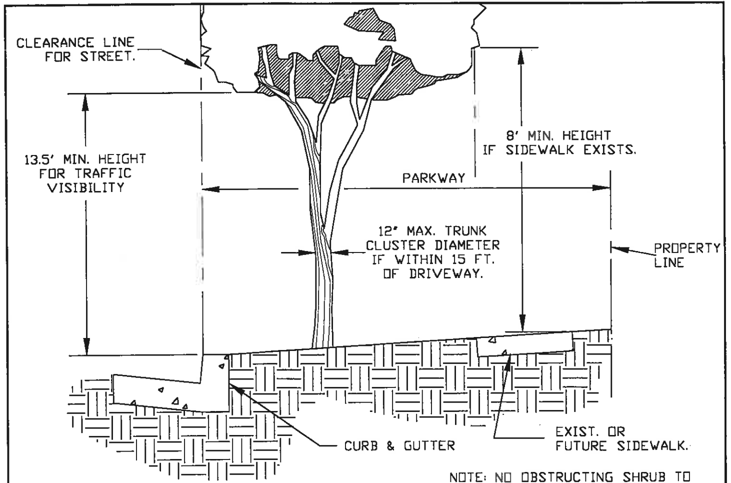
CROSS SECTION
